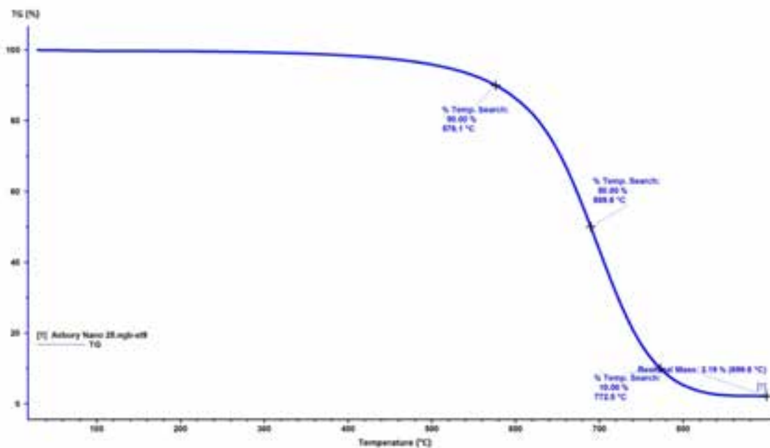
Thermogravimetric curve of GPL graphene nanoplatelets (GrapheneTech).
