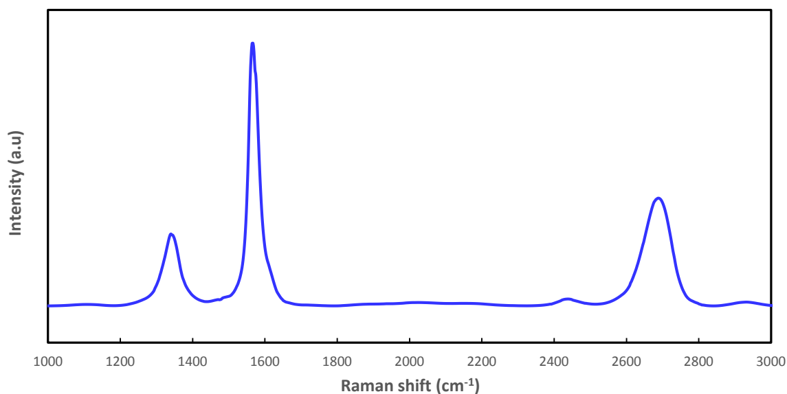
Raman patterns of GPL graphene nanoplatelets (GrapheneTech).
